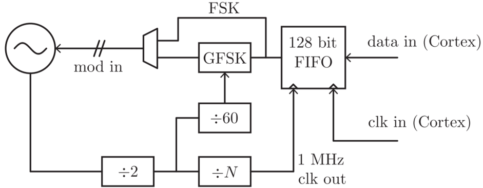
Figure 2.11: BLE modulation schematic as presented in [9].
