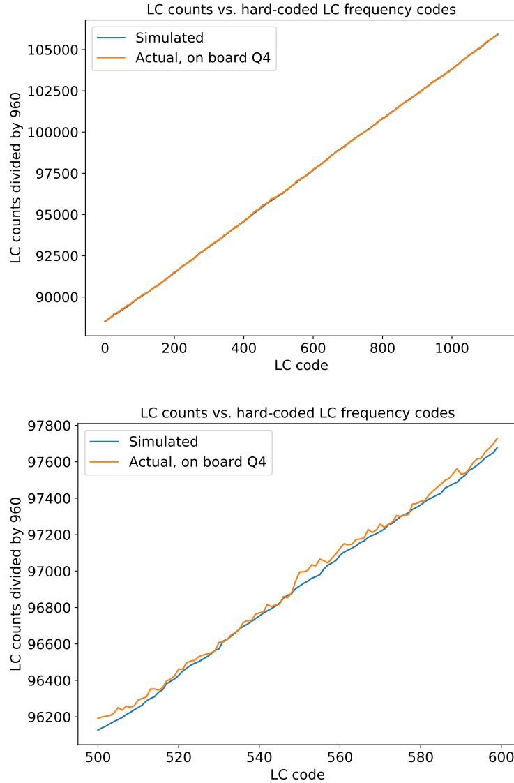
Figure 2.15: LC frequency counts as a function of the 1,133 hard-coded LC monotonic frequency codes, such that the difference between successive codes is at least 8 counts in simulation. The LC counts were recorded once every 40 ms for every LC code.
