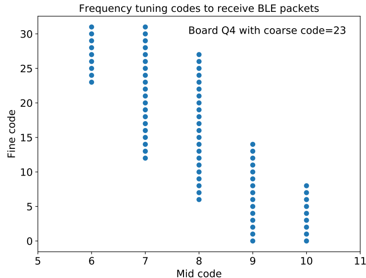
Figure 5.2: The LC frequency codes on SC \mu M development board Q4 on which we could receive BLE packets from board QX7.
