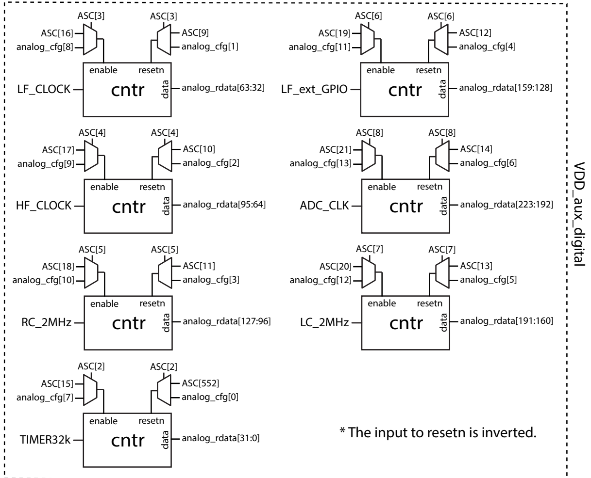
Figure 2.5: On-chip oscillator counters on SC_{\mu}M3C .
