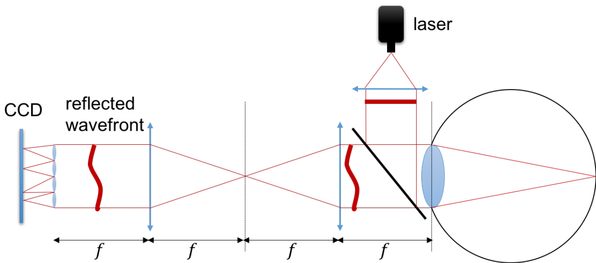
Figure 3.5: wavefront aberrometer.
