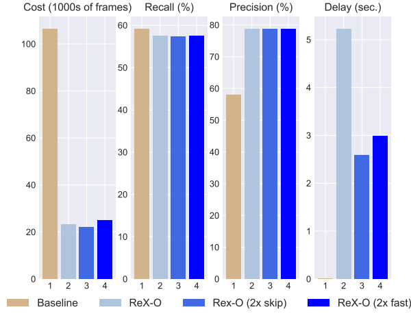
Figure 4.8: Fast-replay search evaluation. Schemes compared: baseline, ReXCam-O (no fast-replay), ReXCam-O (2× skip), ReXCam-O (2× fast-forward). We find that scheme 2× skip outperforms 2× fast-forward on both compute cost and delay reduction.
