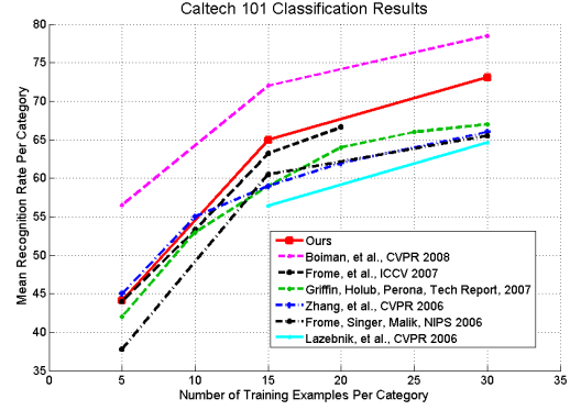
Figure 9. Mean recognition rate (%) over number of training images per category in Caltech 101. With 15 and 30 training images per category, our method outperforms [14, 15, 33, 13] and [19] but [5].
