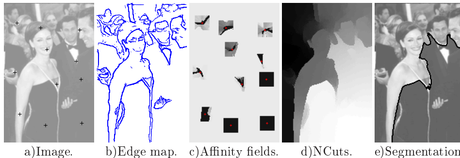
Figure 1: Segmentation by graph partitioning. a) 200 \times 129 image with a few pixels marked(+). b) Edge map extracted using quadrature filters. c) Local affinity fields of marked pixels superimposed together. For every marked pixel, we compute its affinity with its neighbours within a radius of 10. The value is determined by a Gaussian function of the maximum magnitude of edges crossing the straight line connecting the two pixels [9]. When there is a strong edge separating the two, the affinity is low. Darker intensities mean larger values. d) Solution by graph partitioning. It is the second eigenvector from normalized cuts [15] on the affinity matrix. It assigns a value to each pixel. Pixels of similar values belong to the same group. e) Segmentation by thresholding the eigenvector with 0. This gives a bipartitioning of the image which corresponds to the best cuts that have maximum within-region coherence and between-region distinction.
